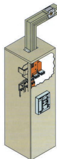
与低压柜可直接对接 Connect directly with Siemens low-voltage switchgear
